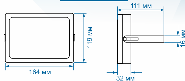
SkatLED LL-30m
