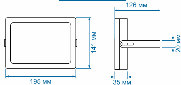
SkatLED LL-30m
